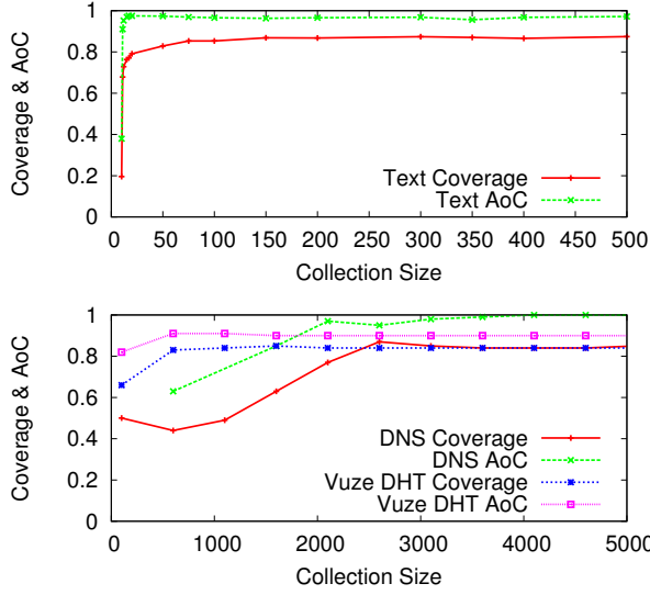
Fig. 8. Coverage and AoC versus the number of conversations. text-based protocol (top); DNS and Vuze DHT binary-based protocols (bottom).
